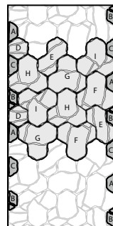
Sidewalk Installation Pattern
