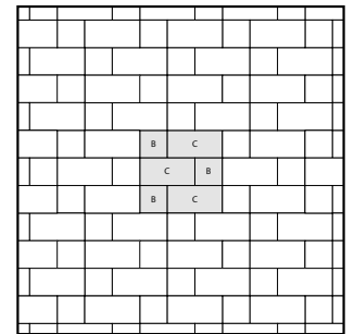
B & C Units Pattern #8 B-33% C-67%
